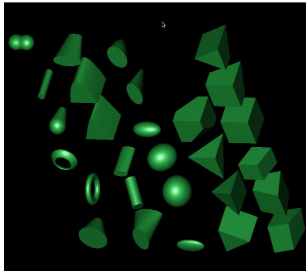
Fig. 1 Geometric primitives
